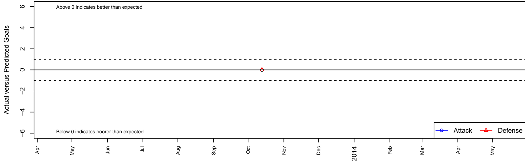
Beach FC Redondo B98 Dots are actual minus expected GF (blue circles) and GA (red triangles). Blue line is smoothed change in attack strength. Red is smoothed change in defense strength.
